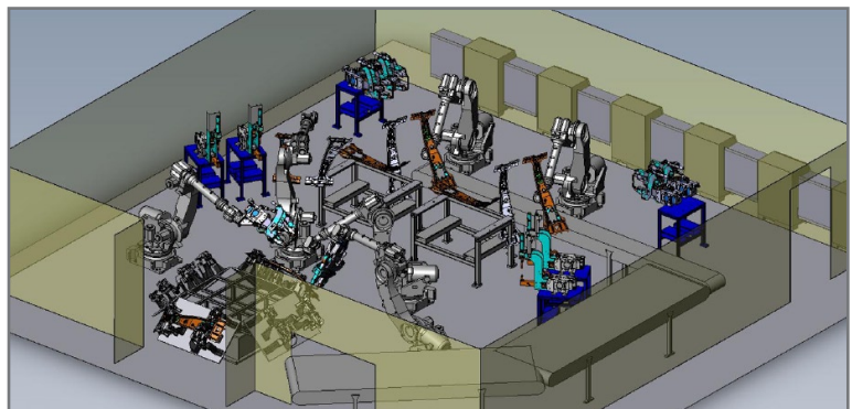
Automated Robotic Resistance Welding Cell
